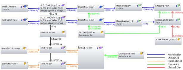
Figure 8 LCA flowchart of scenario with solar panel application
