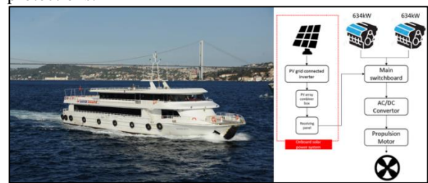
Figure 7 Outline of power distribution for case ship
